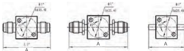
Face seal male (FSR fittings) Face seal swivel male (FSR fittings) Butt welded
